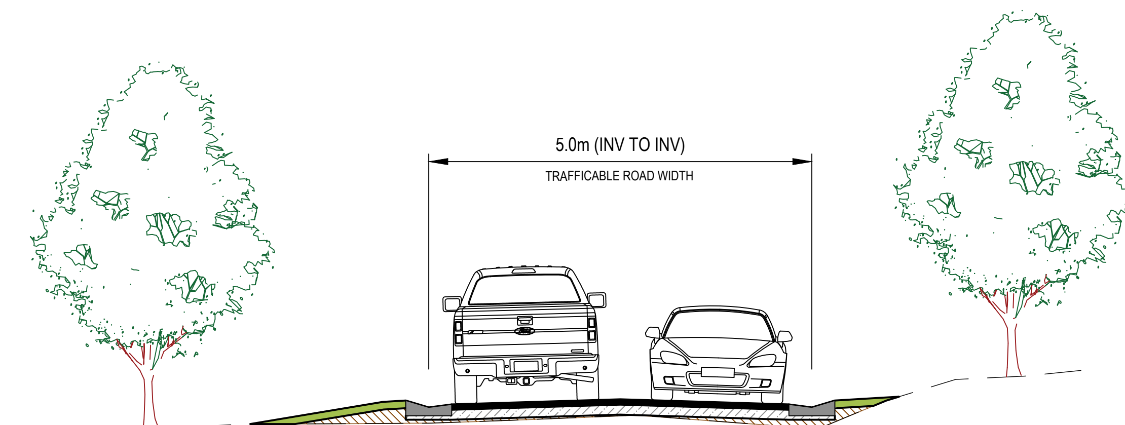
TYPICAL CROSS SECTION - FULL URBAN STANDARD PAVEMENT NOT TO SCALE
