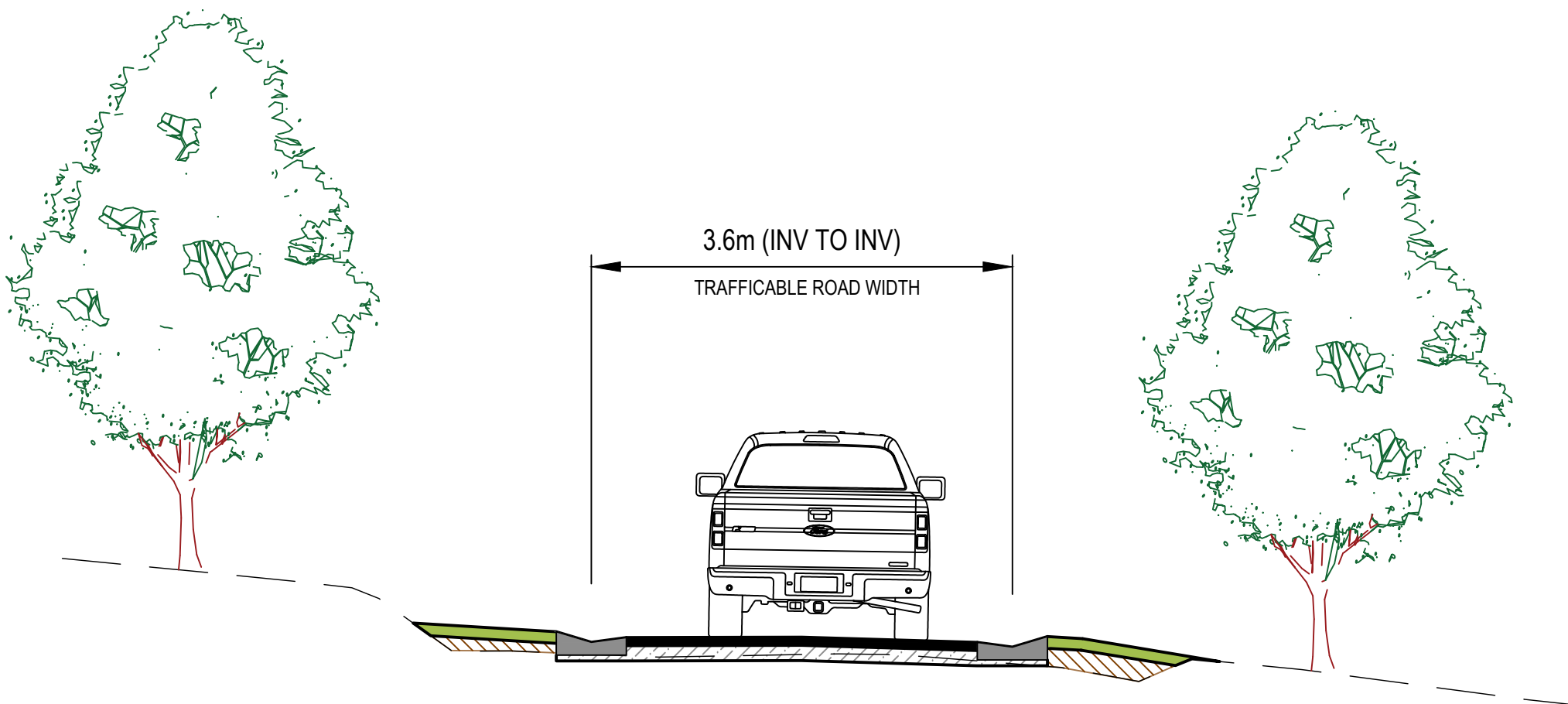
TYPICAL CROSS SECTION - FULL URBAN STANDARD PAVEMENT NOT TO SCALE
