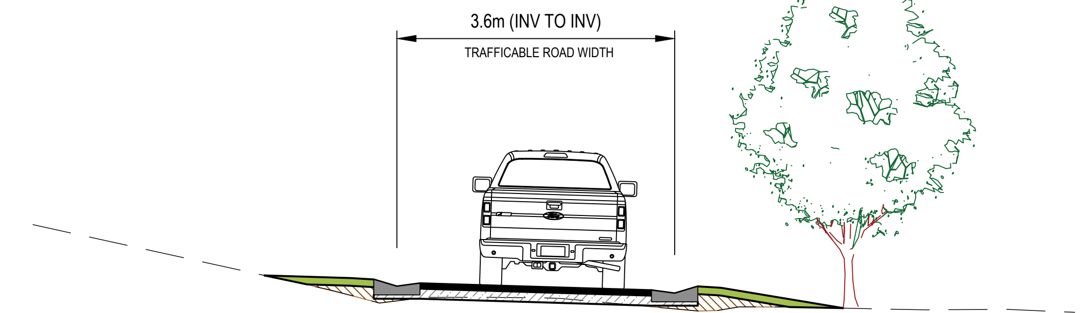
TYPICAL CROSS SECTION - FULL URBAN STANDARD PAVEMENT NOT TO SCALE
