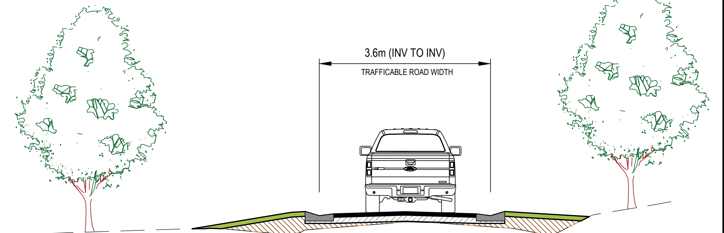
TYPICAL CROSS SECTION - FULL URBAN STANDARD PAVEMENT NOT TO SCALE
